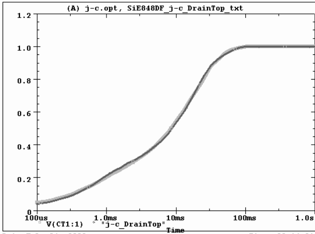
SiE848DF Tank j-c DrainTop Temperature:27.0
