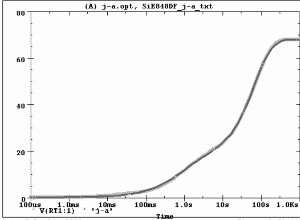
SiE848DF Tank j-a Temperature:27.0
