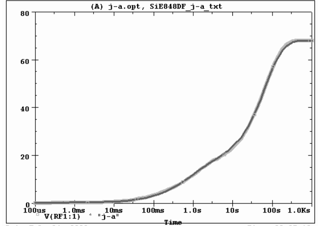
SiE848DF Filter j-a Temperature:27.0
