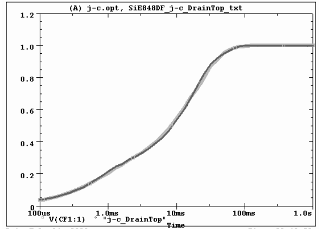
SiE848DF Filter j-c DrainTop Temperature:27.0
