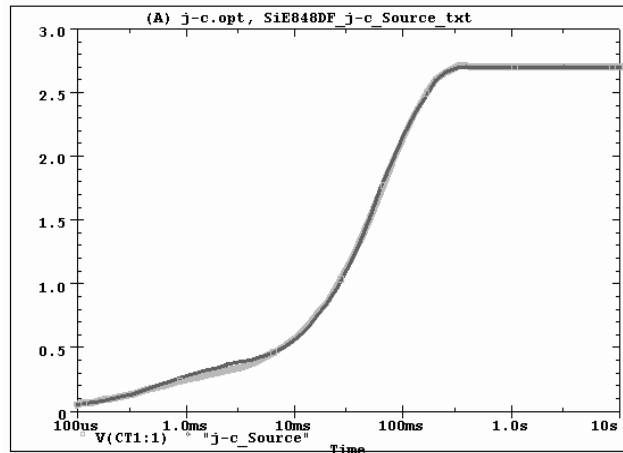
SiE848DF Tank j-c Source Temperature:27.0
