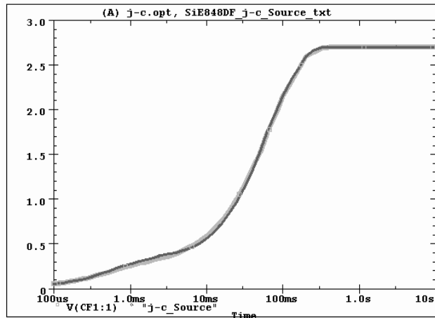
SiE848DF Filter j-c Source Temperature:27.0
